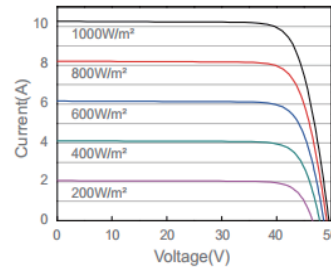
Current-Voltage Curve NUSA144H-440MB
