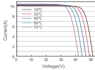
Current-Voltage Curve NUSA144H-440MB
